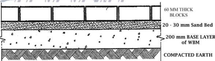
A TYPICAL CROSS SECTION OF BLOCK PAVEMENT USED IN SIDEWALKS / FOOT-PATHS / CAR-PARKS / CYCLE TRACK
