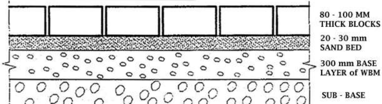
A TYPICAL CROSS SECTION OF BLOCK PAVEMENT USED FOR HEAVILY TRAFFICKED ROADS
